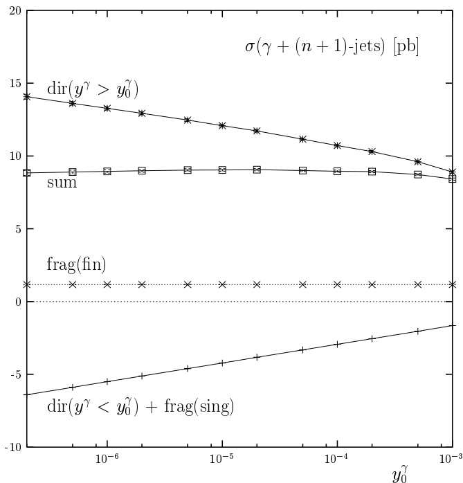
Fig. 1. y_0^\gamma -dependence of separate contributions to the \gamma + (n+1) -jets cross section
