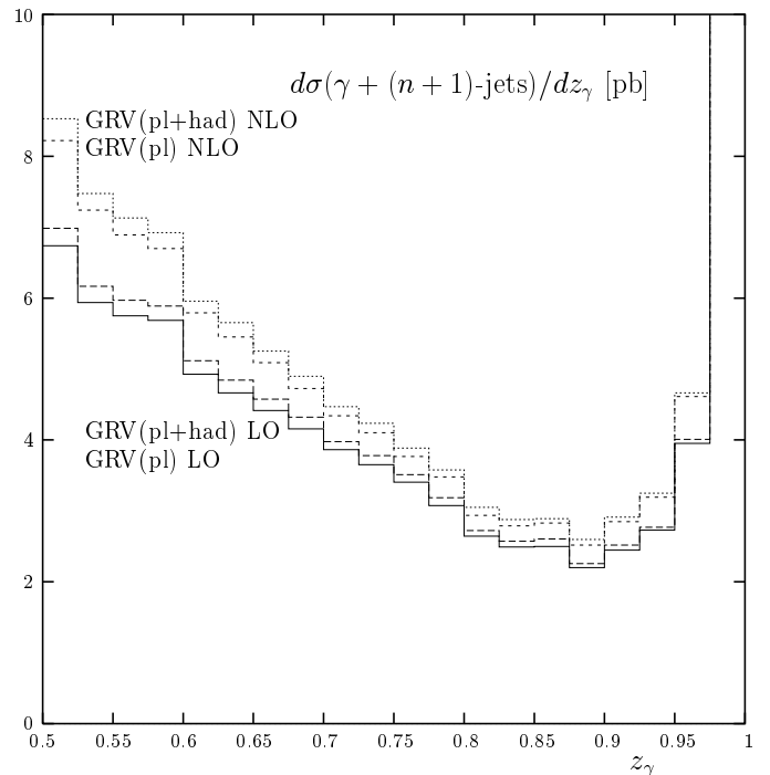
Fig. 4. Comparison of the \gamma + (n+1) -jet cross section for LO and NLO parametrizations of GRV
