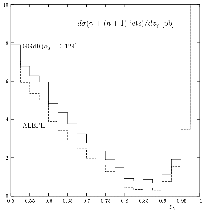
Fig. 2. Comparison of the \gamma + (n+1) -jet cross section for the LO and NLO parametrizations of the FF obtained from fits to the ALEPH data
