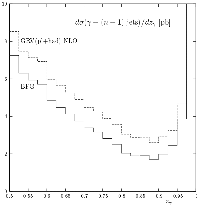
Fig. 3. Comparison of the \gamma + (n+1) -jet cross section for the NLO parametrizations of GRV and BFG
